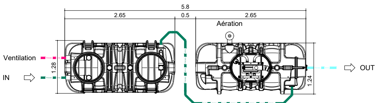
X-PERCO R-90 5 EH (bi-cuves)
