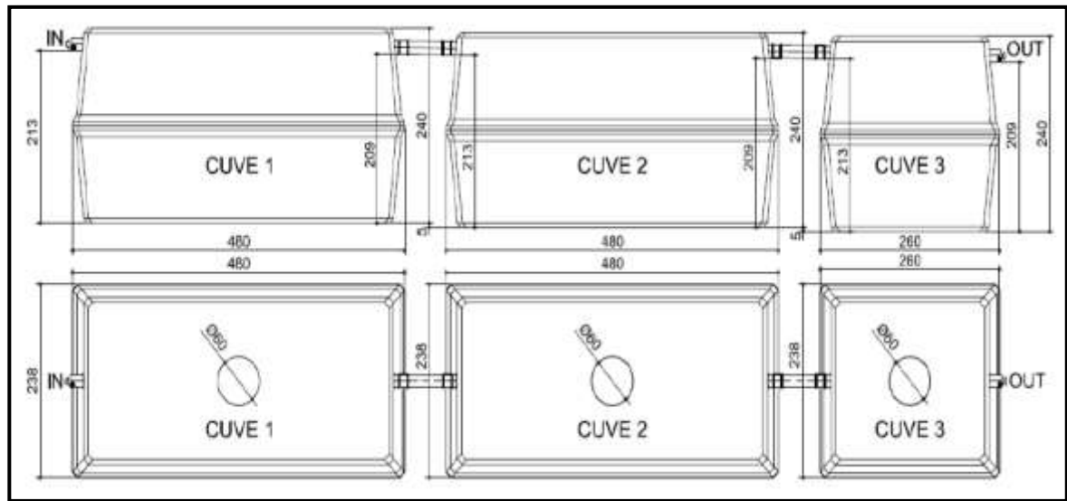
Fig-16 : Dimensional drawing of the Oxyfix® C-90 CB 76-99 PE
