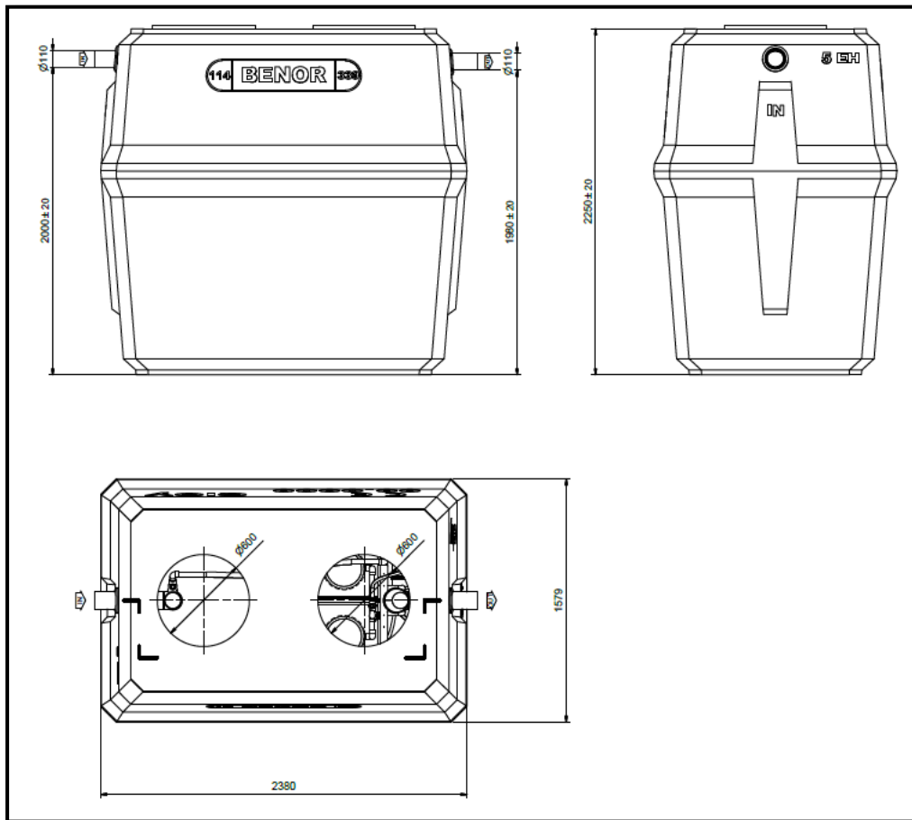
Fig-8 : Dimensional drawing of the Oxyfix C-90 MB 5 et 6 PE
