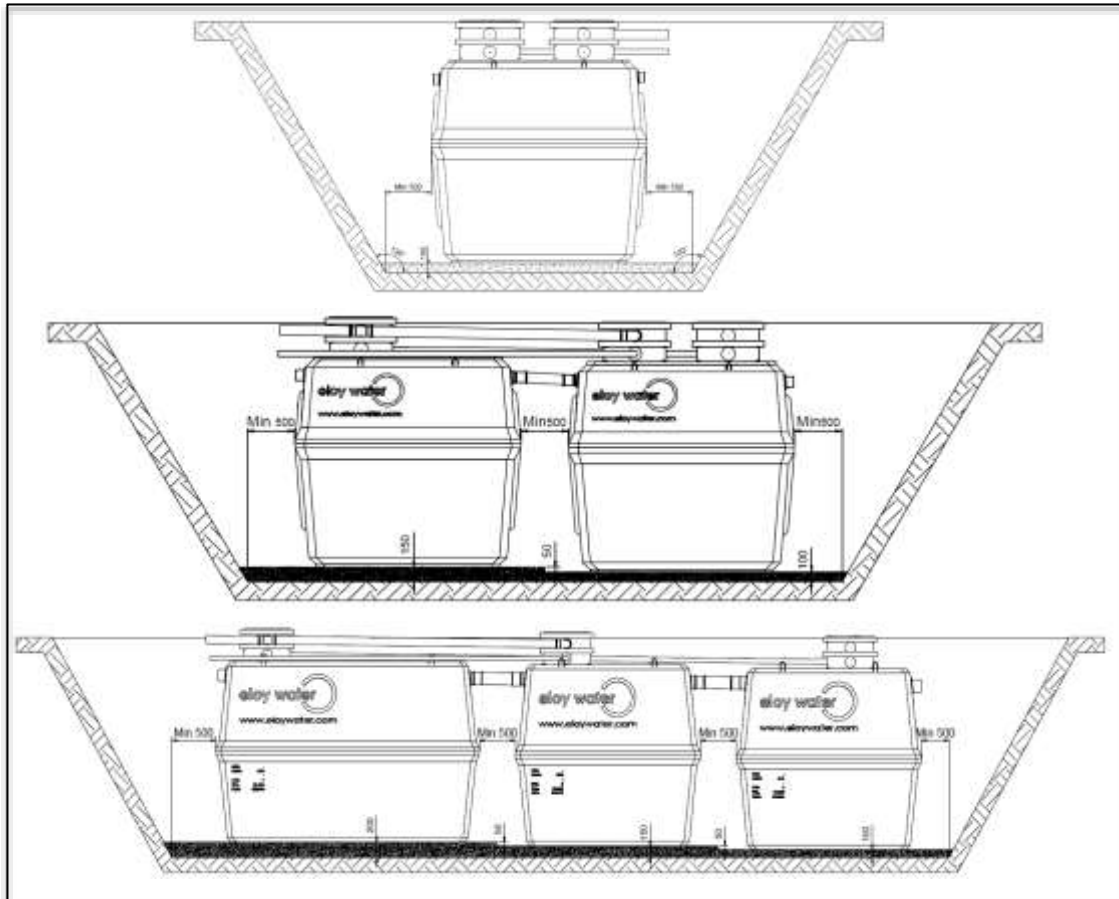
Fig-19 : Layout drawing of the unit
