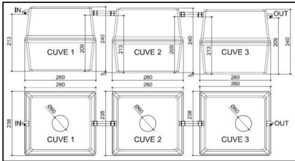
Fig-13 : Dimensional drawing of the Oxyfix® C-90 CB 28-38 PE
