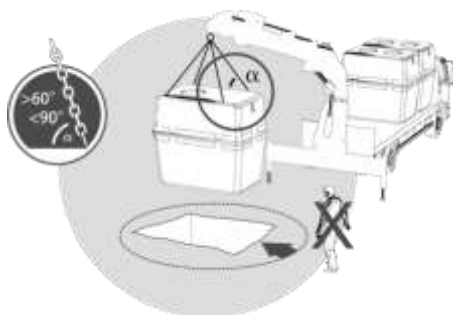
Fig-17: Handling the C-90 tank
