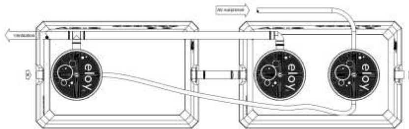
Fig-24: Vent pipe fitted to a two-tank Oxyfix® C-90 unit
