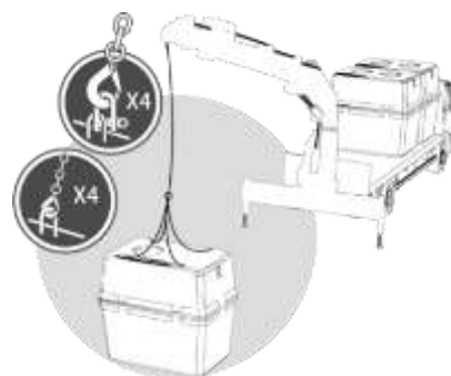
Fig 18: Handling the C-90 tank
