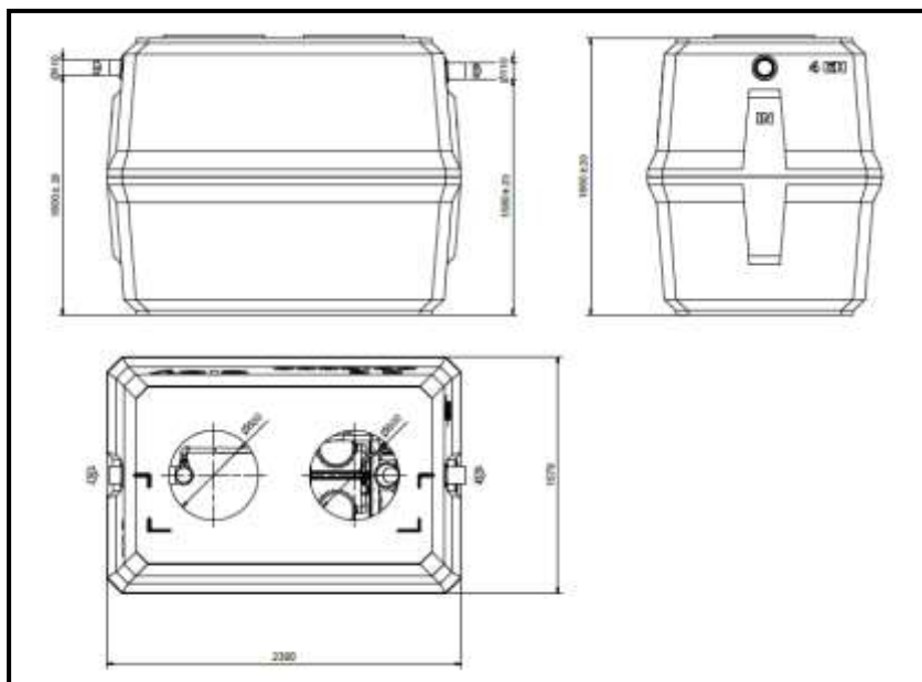
Fig-7 : Dimensional drawing of the Oxyfix C-90 MB 1-4 PE (1)
