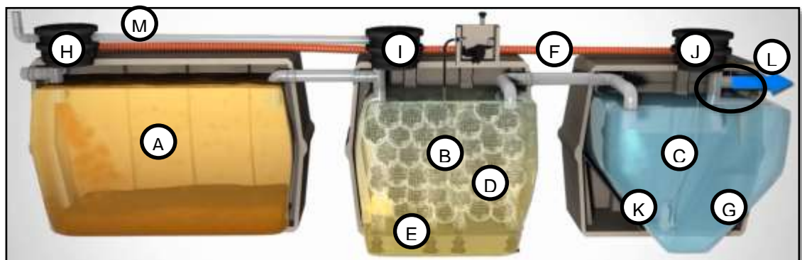
Fig-5: Pictorial diagram of the Oxyfix® C-90 Three Tank Unit
