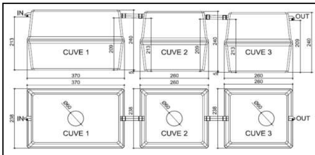
Fig-14 : Dimensional drawing of the Oxyfix® C-90 CB 39-58 PE
