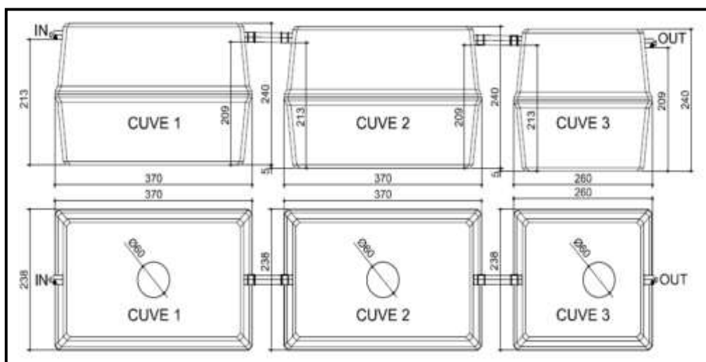
Fig-15 : Dimensional drawing of the Oxyfix® C-90 CB 59-75 PE
