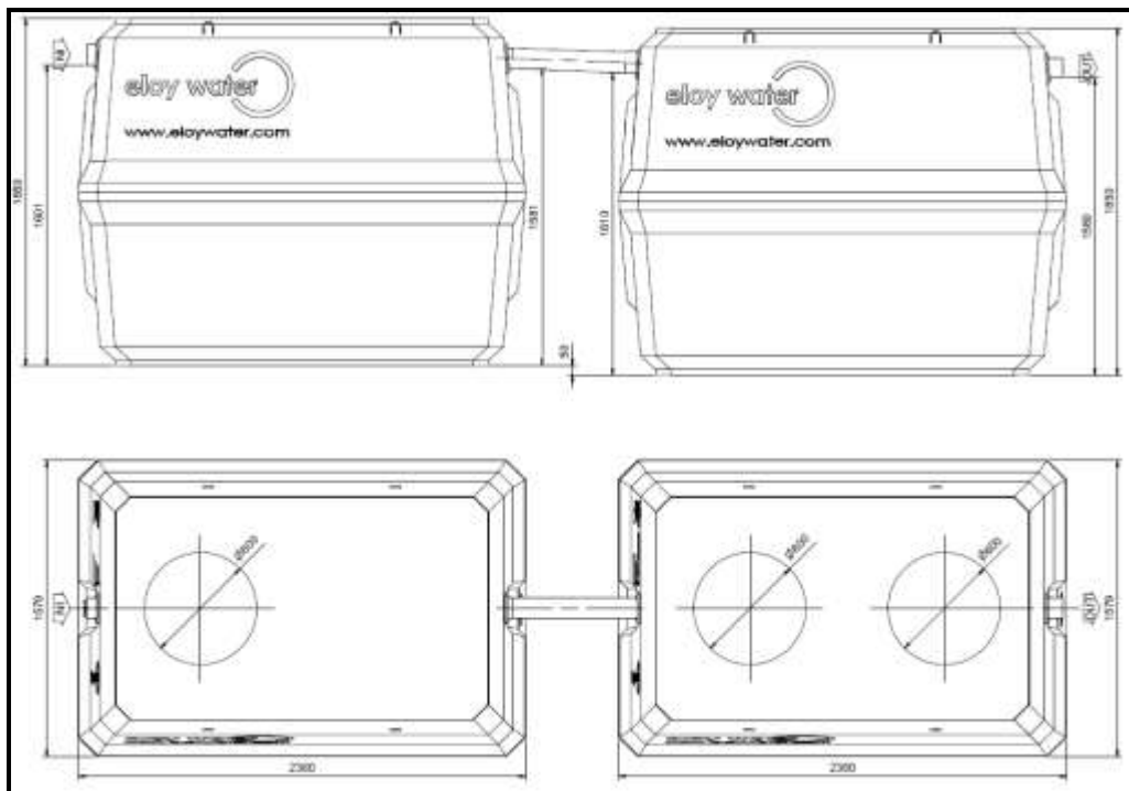
Fig-9 Dimensional drawing of the Oxyfix® C-90 MB 7 PE
