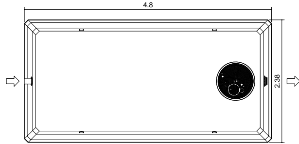
WATERBUFFER C-90 20 m 3 - Buffer 2.4 m 3
